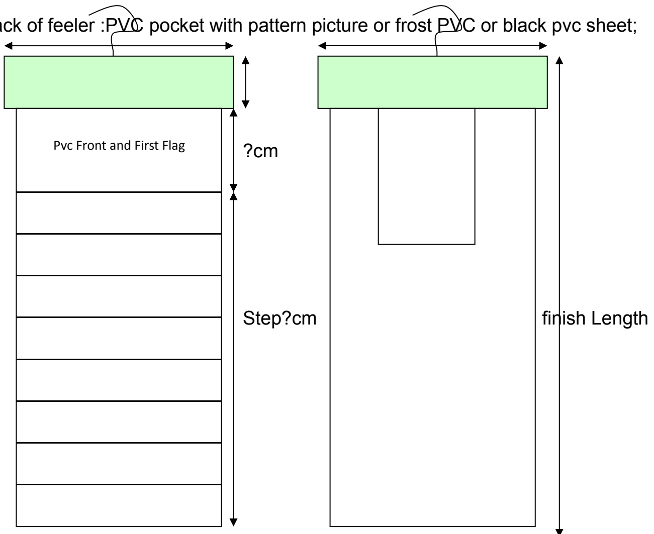
Hanger front
